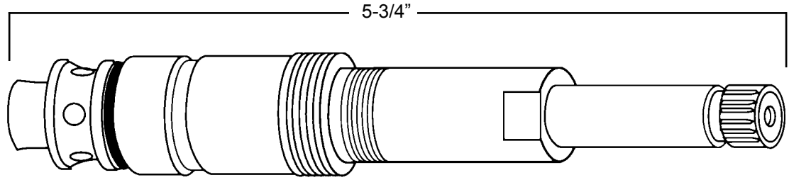
43411 Long pattern Colony transfer stem assy.
