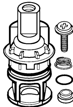
46120 Ceramic cartridge for HDF faucets
