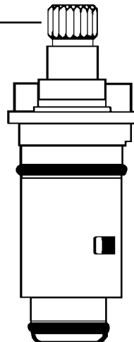
Short cartridge assy. 49005 Cold 49006 Hot
