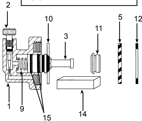
FOOT VALVE REPAIR KIT
