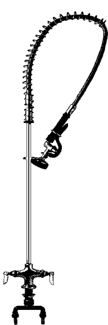
25603 pre-rinse unit -4" center deck -under sink 1/4" IPS tailpieces -approx. 48" high -15" overhang
