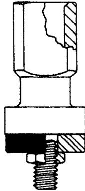
95113 Zurn old style plunger
