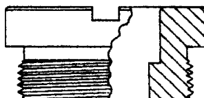
94408 Smith wall hydrant face nut
