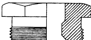
95053 brass 95054 chrome Wade, Josam, Prier stem bushing nut
