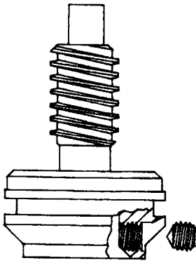
95006 Josam actuator for Hydrasan I & II 11544 o-ring 22014 key
