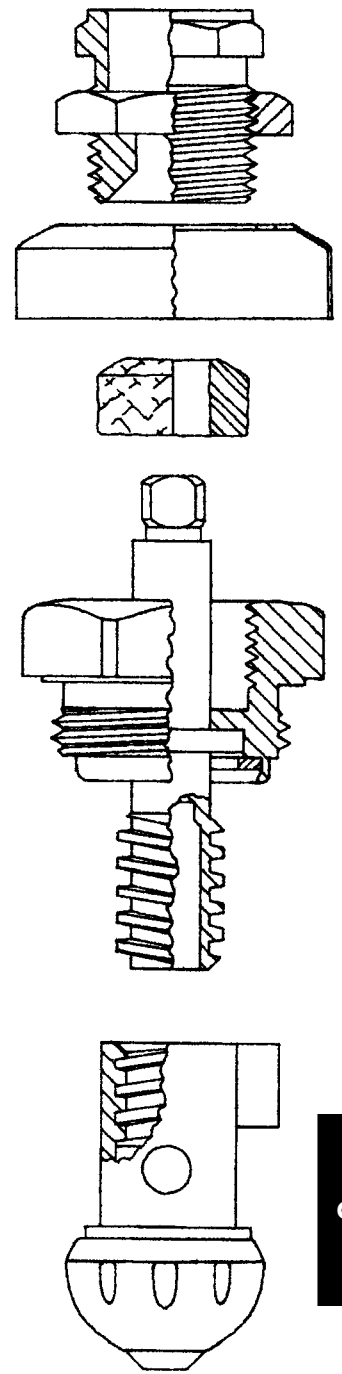
95003 replacement for Woodford #RK-71
