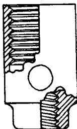
95101 Smith old style fine thread block
