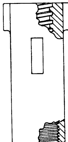
94109 Woodford yoke nut
