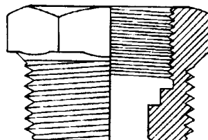
95050 brass 95051 chrome Wade, Josam, Prier worm nut
