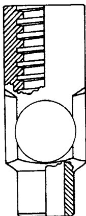
95107 3/8" sweat worm sleeve
