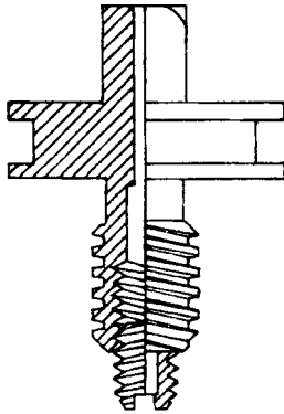
95003A combination operating screw & relief port 11572 o-ring 22016 key
