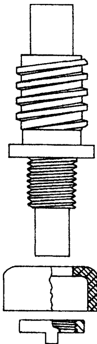
95033 Eclipse old style operating stem
