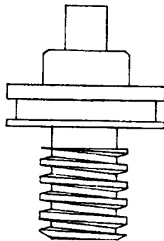
95002 coarse thread operating screw 11569 o-ring 22015 key
