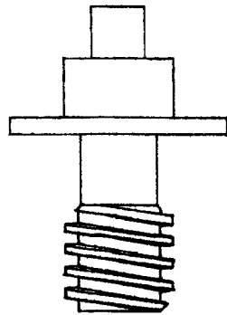
95030 Smith coarse thread operating screw 22015 key
