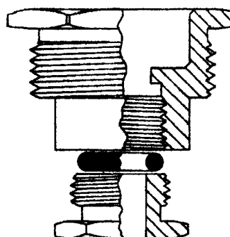
95061 replacement Josam model Y-210 head nut
