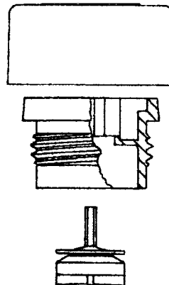
94403 Nibco model #90 frost free vacuum breaker kit
