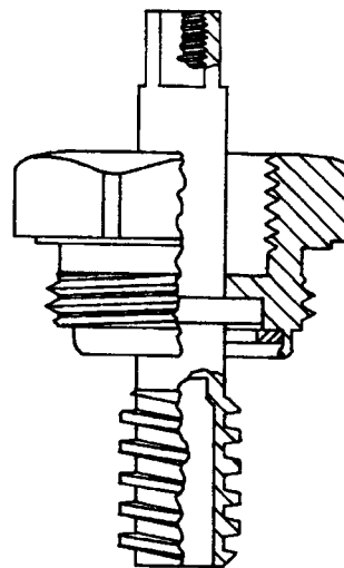
94059 Woodford head nut assembly
