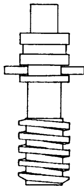
95004 Wade, Prier operating screw 11508 o-ring 22015 key
