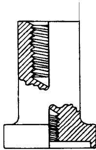
95000 Smith plunger
