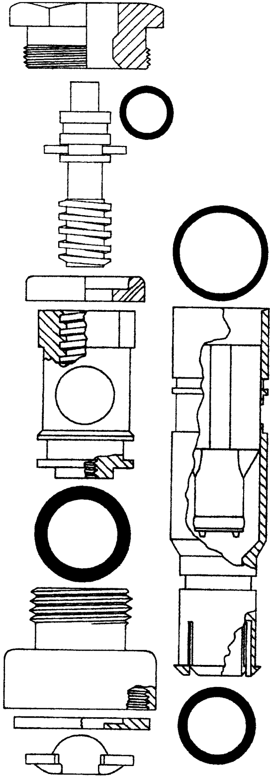
95369 replacement for Wade #WKO4
