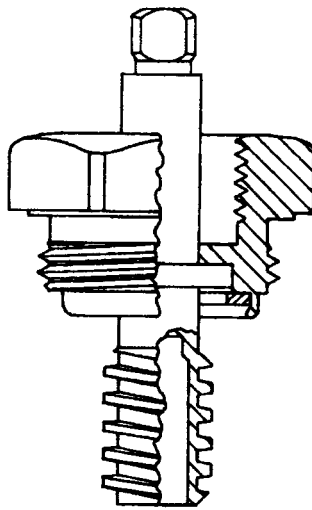
94110 Woodford head nut assembly
