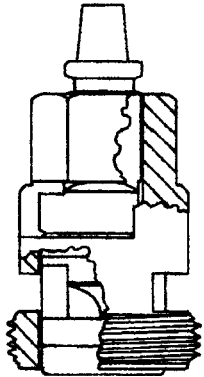
94589 valve body assy. retaining ring valve body valve actuator nylon thrust washer rotating ceramic disc fixed ceramic disc silicon rubber seal retainer guide
