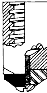
95020 Wade plunger
