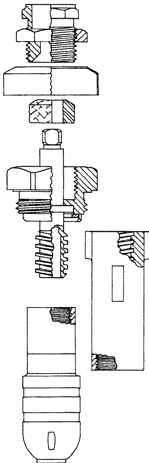
95003 replacement for Woodford #RK-Y95
