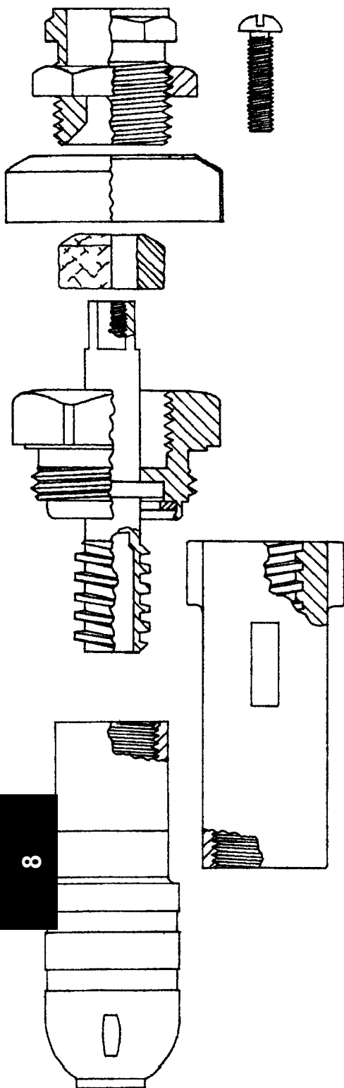
95001 replacement for Woodford #RK-Y30
