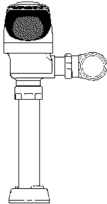
G2 closet flushometer complete
