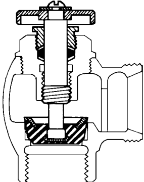
3/4" angle stop
