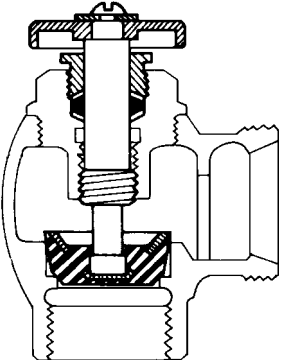
1" angle stop
