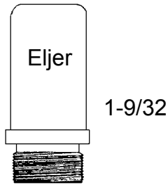
1-9/32 1/2-27 thrd 12073 brass
