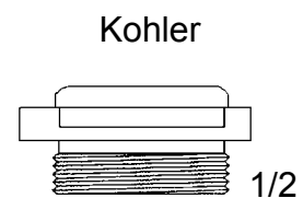
1/2 53/64-24 thrd 12118 brass
