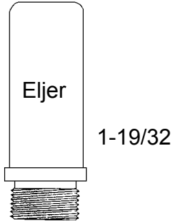
1-19/32 1/2-27 thrd 12074 brass
