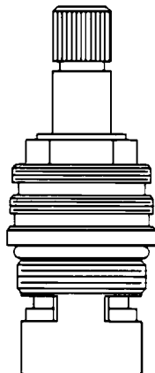
2-5/16" short cartridge 48902 Cold 48901 Hot
