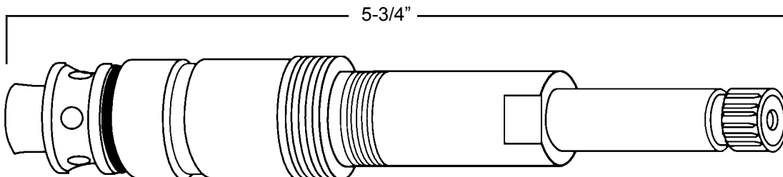
43411 Long pattern Colony transfer stem assy.
