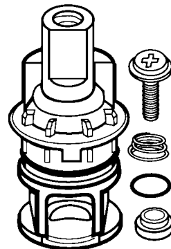
46120 Ceramic cartridge for HDF faucets
