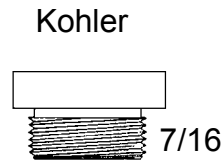
7/16 9/16-20 thrd 12112 brass
