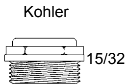
15/32 11/16-27 thrd 12120 brass
