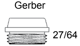
27/64 5/8-20 thrd 12080 brass 13080 monel
