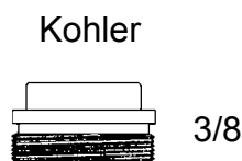
3/8 5/8-27 thrd 12115 brass 13115 monel
