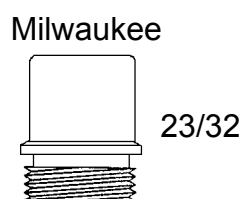
23/32 33/64-27 thrd 12130 brass
