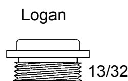
13/32 5/8-27 thrd 12125 brass 13125 monel
